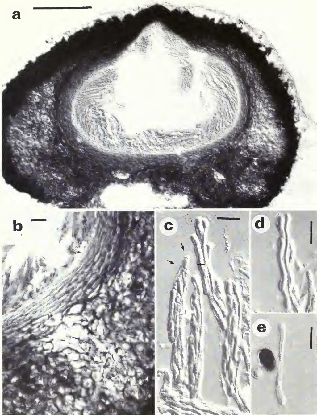
Fig. 55 Sarcopyrenia gibba (Nyl.) Nyl. (H-NYL 4058—lectotype) (a) Vertical section of ascoma; scale = 100 \mu m; (b) Detail of wall layers: textura angularis and textura somewhat prismatica, with cells compressed laterally; (c) Ascus and ascospores, arrows showing faint ascus wall; (d), (e) Ascospores; scale = 10 \mu m.
